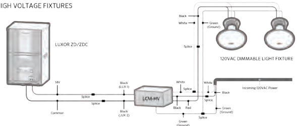
[C] HIGH VOLTAGE FIXTURES
